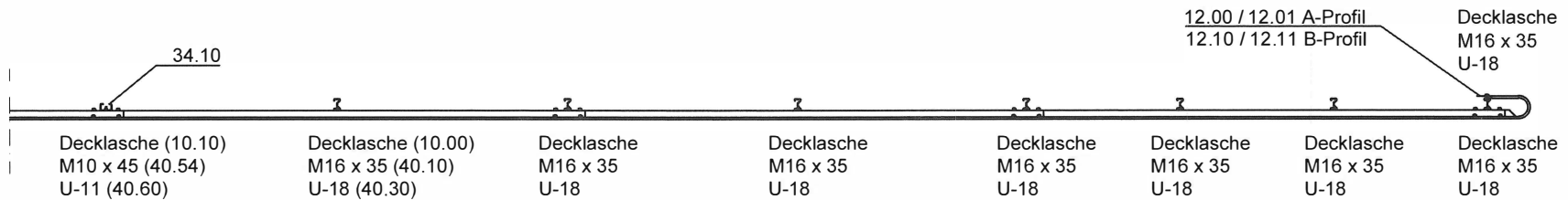
Detail X
