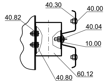
Detail X
