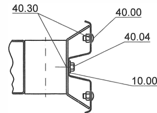
Detail X
